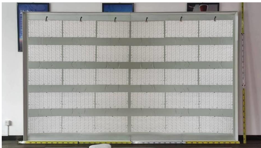
Internal view of CS-LBPF-RGBW-960-24
