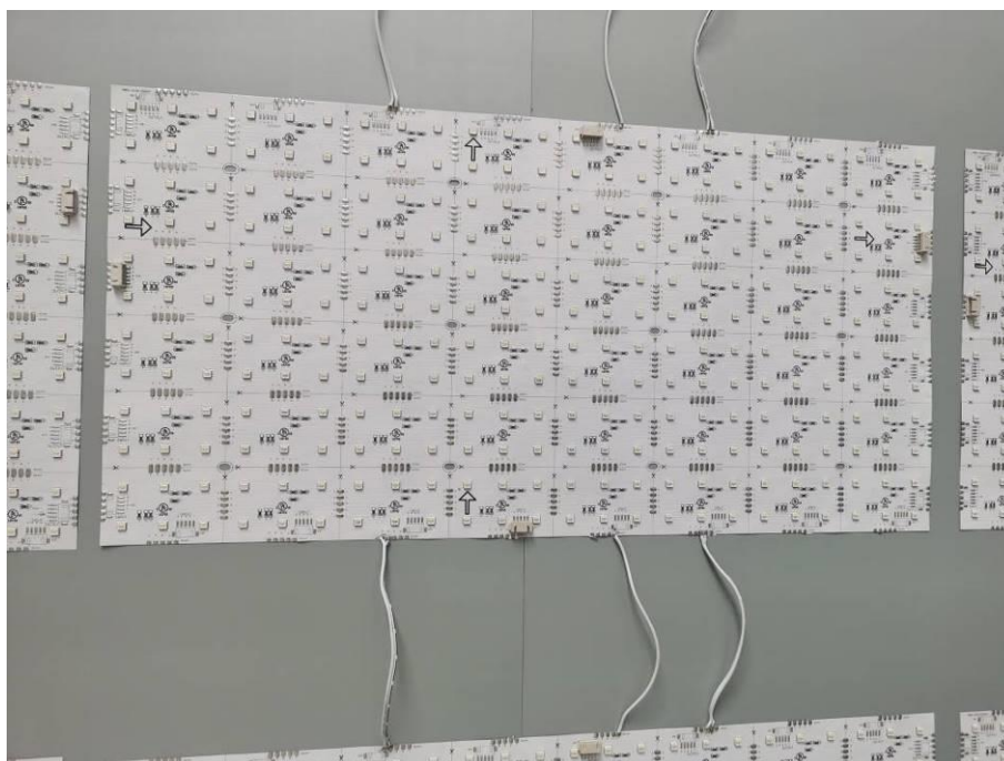
LEDs view of CS-LBPF-RGBW-960-24
