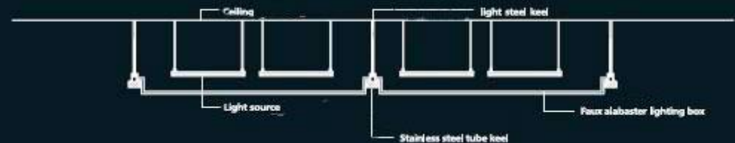
The installation of faux alabaster lighting box in the ceiling
