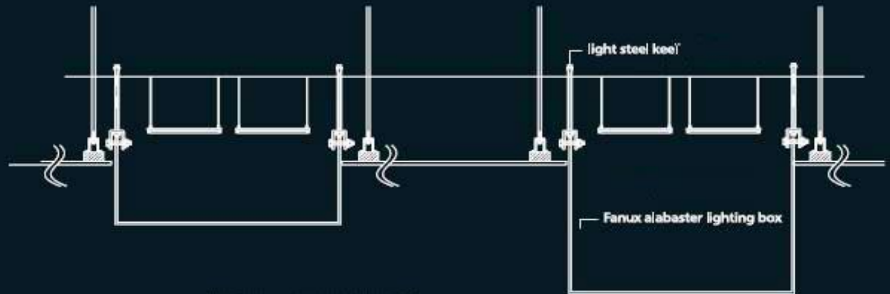
The installation of faux alabaster lighting box in the ceiling
